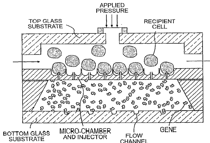
CELL TRANSFORMATION MICRODEVICE
